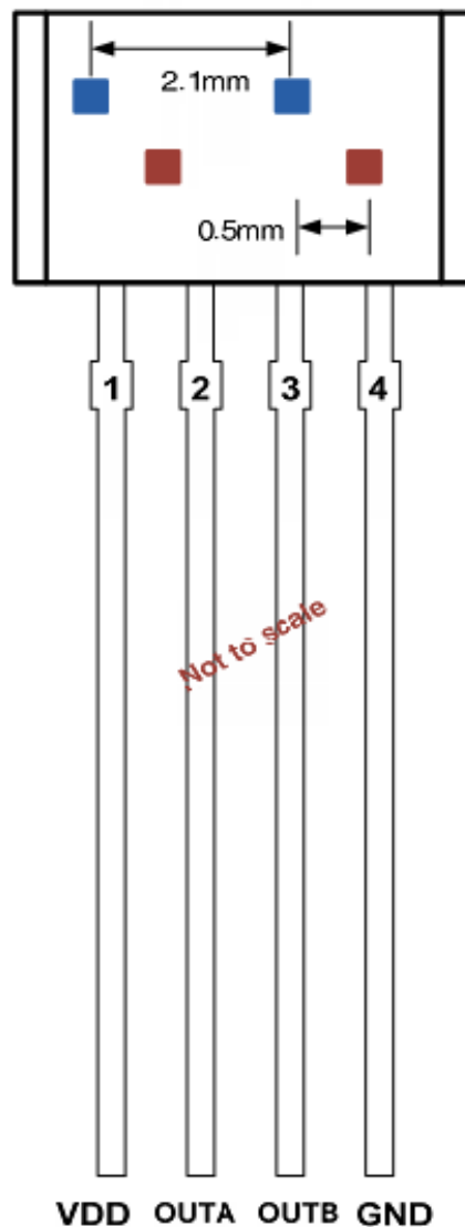
4-Terminal SIP VB package (Top View)
