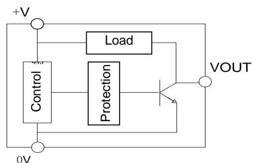
NPN (RC) Output (Pull-up resistor: 3kΩ, customizable)
