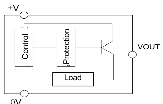
PNP (RC) Output (Pull-down resistor: 3kΩ, customizable)
